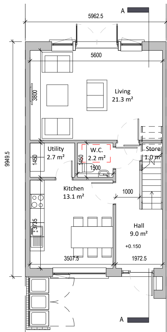
1 Ground Floor 1 : 100
