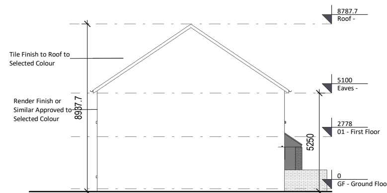
6 Gable Elevation 1 : 200
