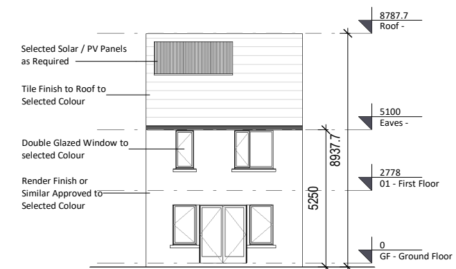
4 Rear Elevation 1 : 200
